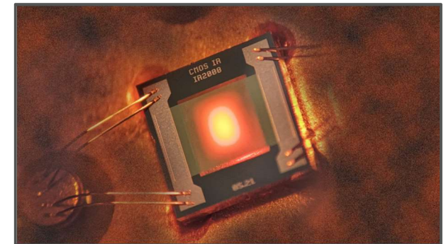
MEMS IR-Strahler
